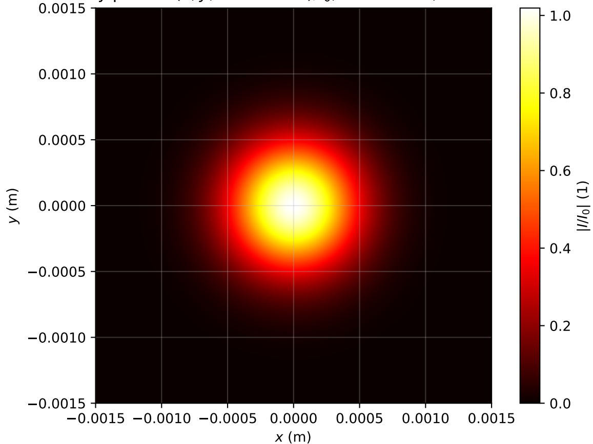
Intensity profile I(x, y, z = 0.159m)/I_0 , Pin=1.0Pcr, artificial time
